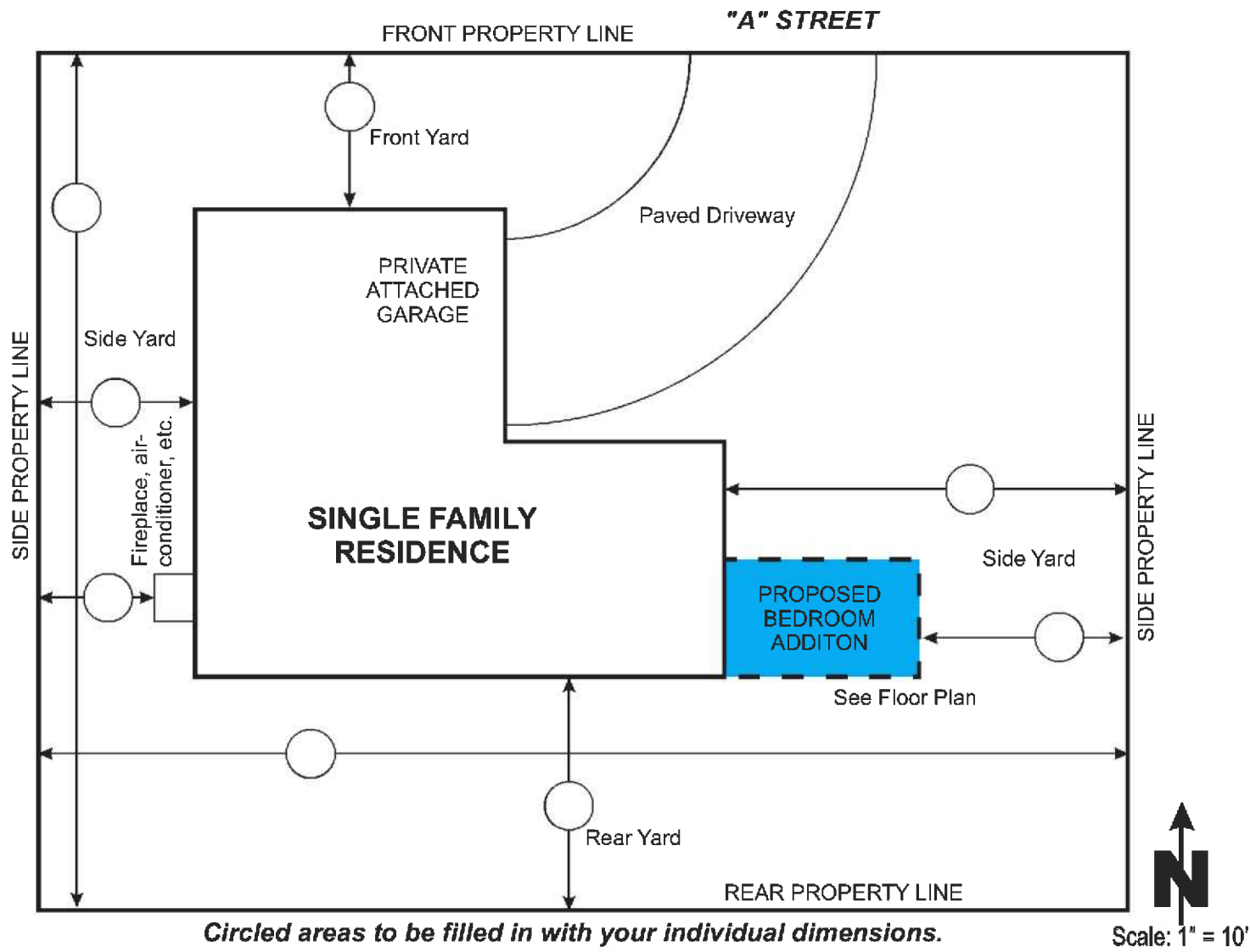
SAMPLE PLOT PLAN (See Minimum Plan Submittal Requirements handout for additional information)
